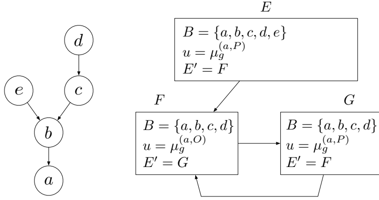
Figure 1: An AF and belief state structure.
