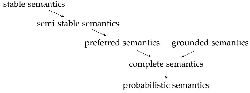
Figure 3: Relationships between semantics
