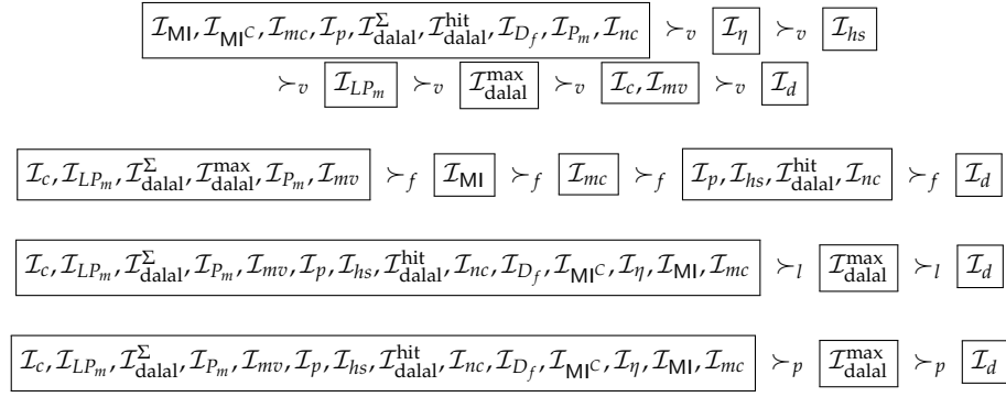
Figure 1: Expressivity orders of the investigated inconsistency measures; measures within the same box are equally expressive wrt. the particular expressivity characteristic
