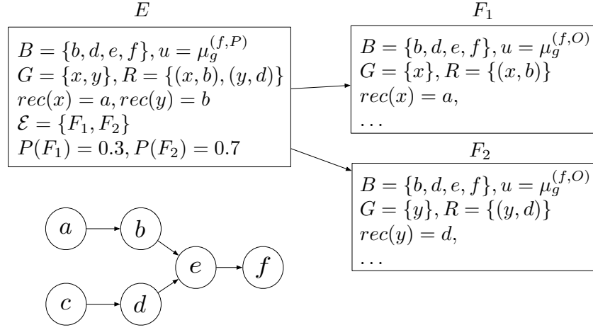
Figure 3: An AF and belief state structure.
