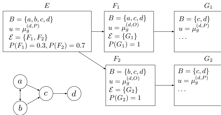
Figure 2: An AF (left) and belief state (right).
