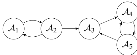
Figure 1: A simple argumentation framework
