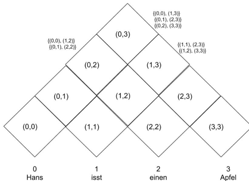
Figure 18: CKY chart
