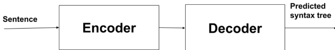
Figure 20: Broad Architecture
