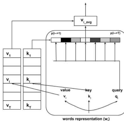
Figure 17: Self-attention module
