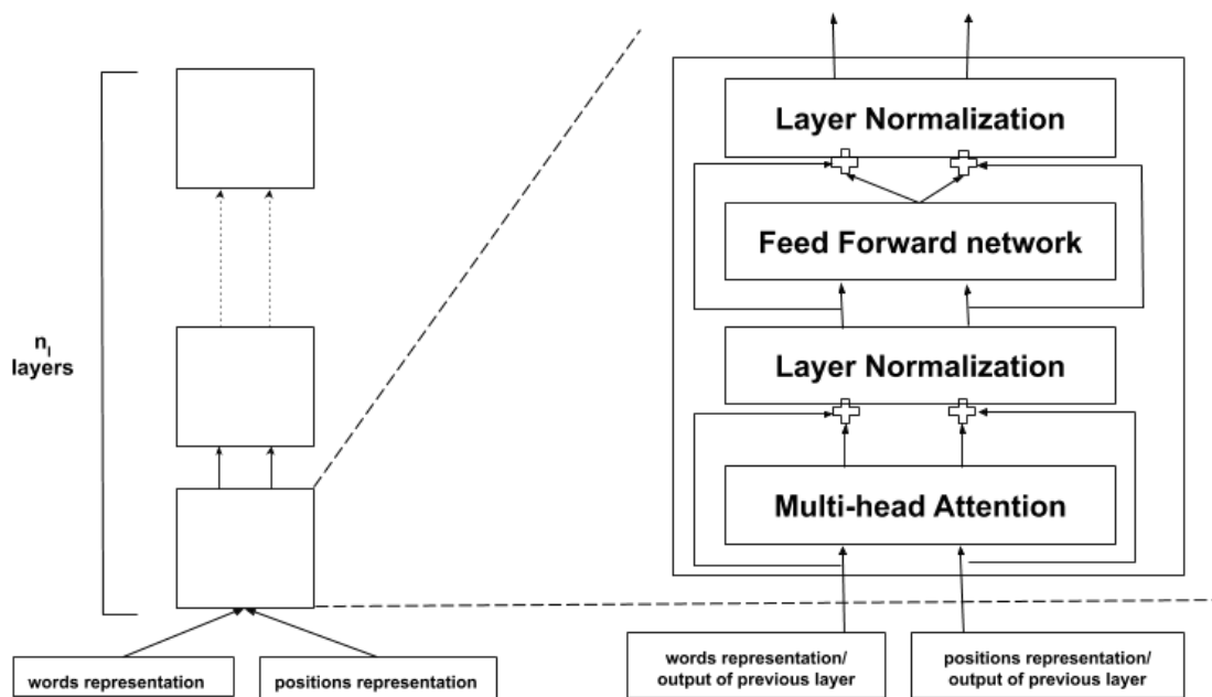
Figure 21: Encoder module
