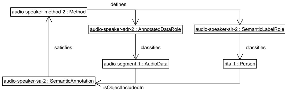
Figure 8: Annotation of a call segment with the speaker Rita
