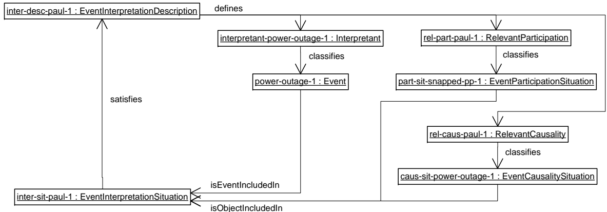
Figure 10: Representing Paul’s interpretation that a snapped power pole has caused the power outage
