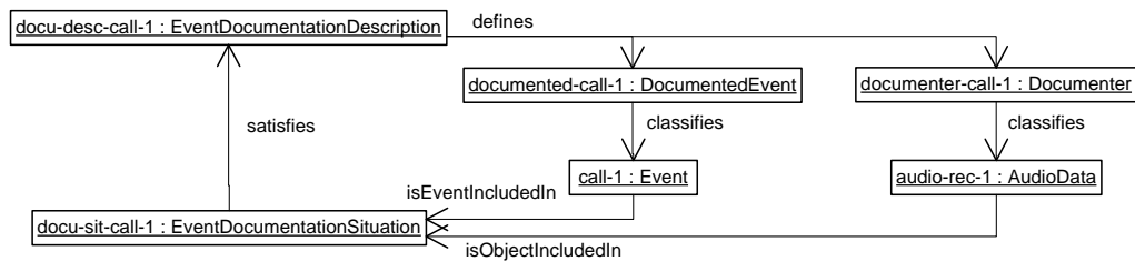
Figure 3: Documentation of Paul's call to the emergency hotline with an audio recording
