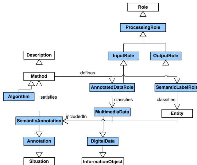
Figure 24: Semantic annotation pattern
