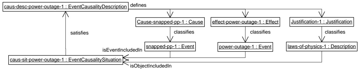
Figure 9: Causal relationship between a snapped power pole and a power outage
