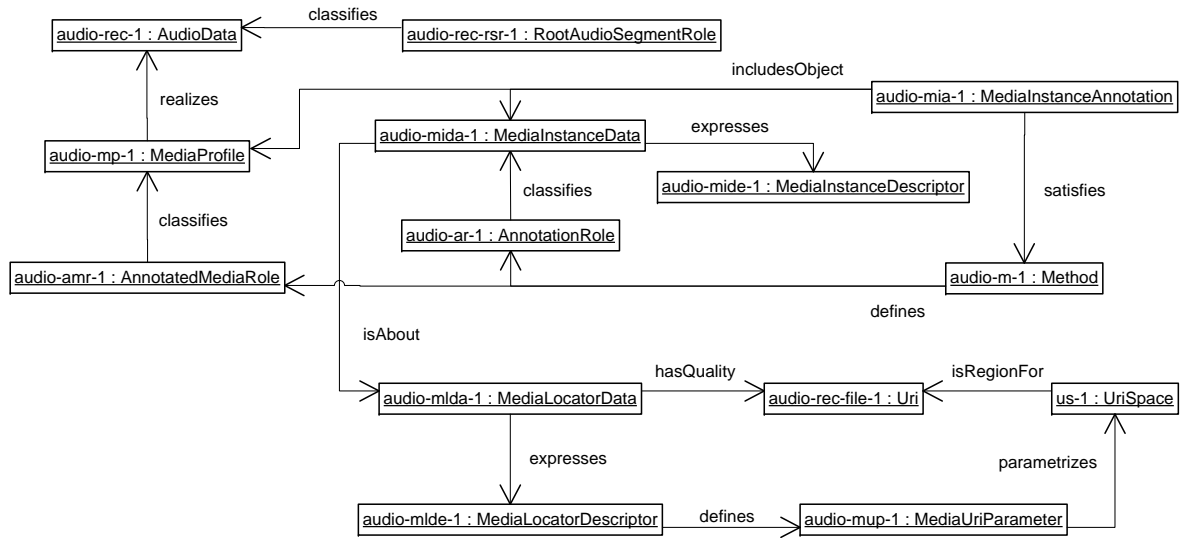
Figure 5: Representation of an audio recording and the file that realizes the recording
