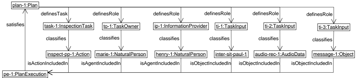
Figure 12: Description of the task sent to Marie
