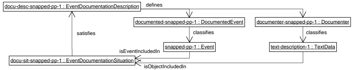
Figure 4: Documentation of the snapped power pole event with textual instructions for the emergency entities
