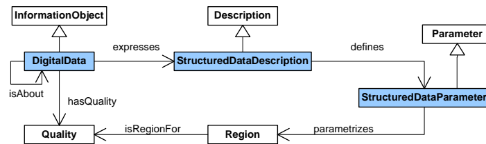
Figure 20: Digital data pattern
