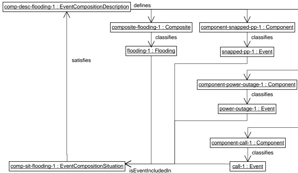
Figure 13: Modeling the large flooding event by composition of smaller events
