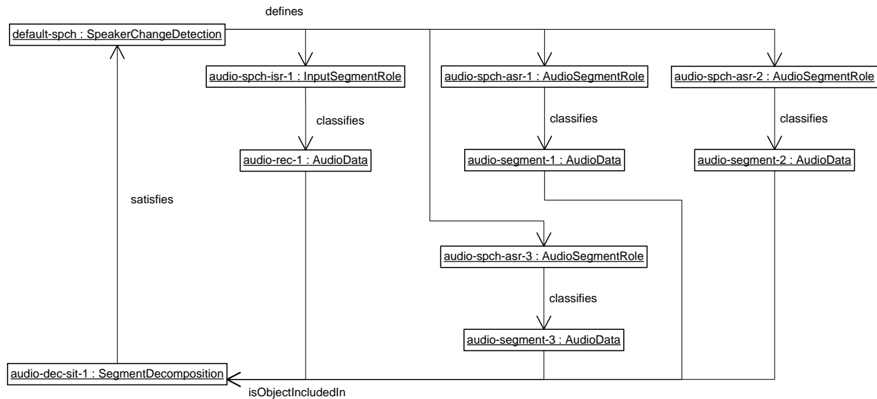
Figure 6: Decomposition of the call recording into segments
