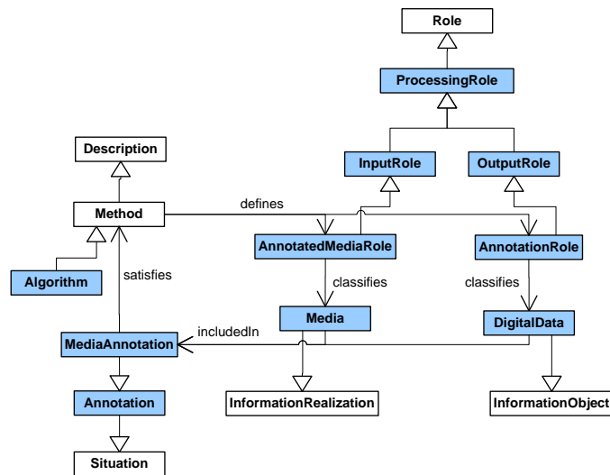
Figure 23: Media annotation pattern
