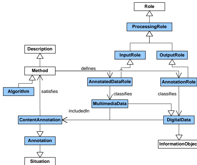
Figure 22: Content annotation pattern
