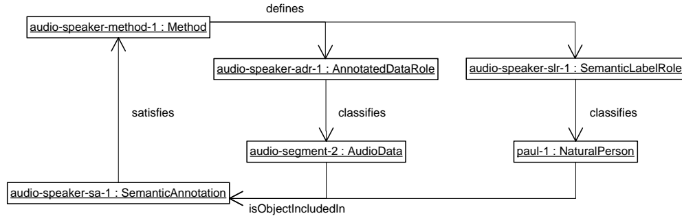
Figure 7: Annotation of a call segment with the speaker Paul
