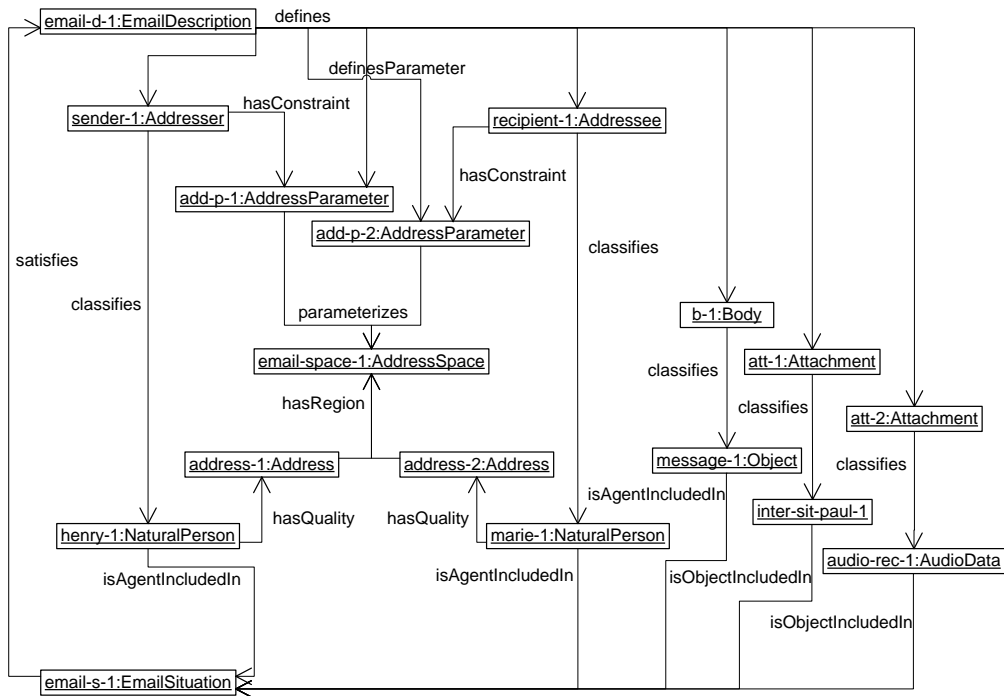
Figure 11: Henry sends Marie a message with a task description
